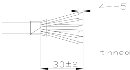
Figure 5.2 USB-RS485-WE Mechanical Details (dimensions in mm)
